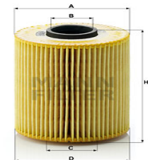
Oil Filter HU 926/4 x EM-10094
