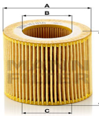
Oil Filter HU 816 z KIT EM-10091
